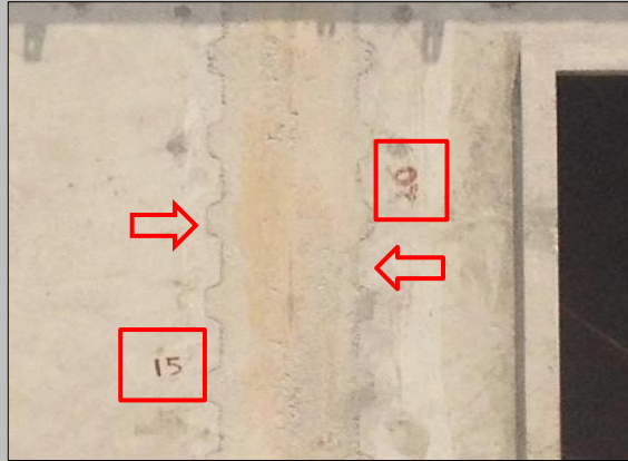
Modular shear keys ( wet joint )
