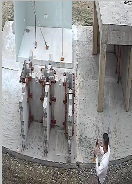
- 23 rd July 2019 Mock-up panel : Inspection on monolithic wall system with modular shear key (wet joint)
